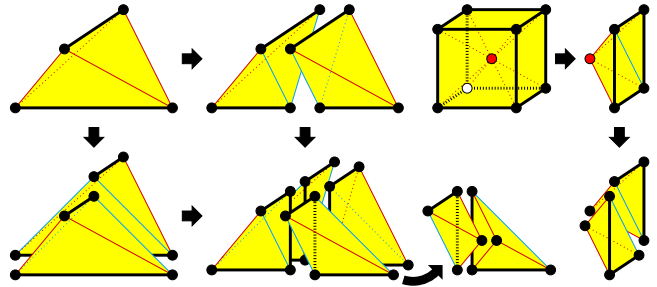
Figure 7: Graded background grids consist of BCC tetrahedra, bisected BCC tetrahedra, quadrisectioned BCC tetrahedra, and half-pyramids.
