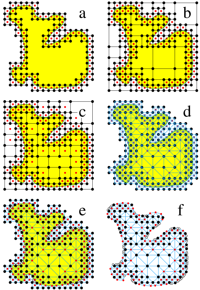
Figure 9: A two-dimensional illustration of the (three-dimensional) algorithm. (a) Cells intersecting the isosurface. (b) After enforcing the Continuation Condition and building an octree. (c) After enforcing the Weak Balance Condition. (d) The background grid. (e) After introducing cut points and warping the vertices. (f) The final mesh.
