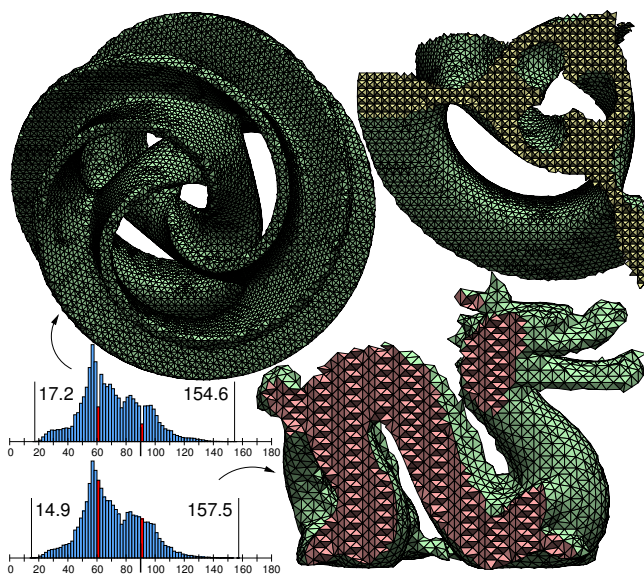
Figure 4: Meshes of uniformly sized tetrahedra produced by isosurface stuffing with \alpha_{\text{long}} = 0.28511 and \alpha_{\text{short}} = 0.39882 . Whirled White Web is by courtesy of Carlo Séquin. Histograms tabulate the dihedral angles in 2^\circ intervals; multiply the heights of the red bars by 20.
