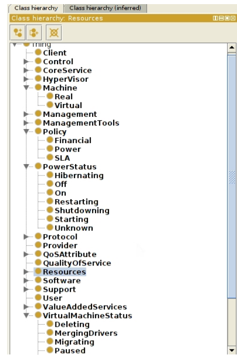
Fig. 1. Proposed Ontology View.
