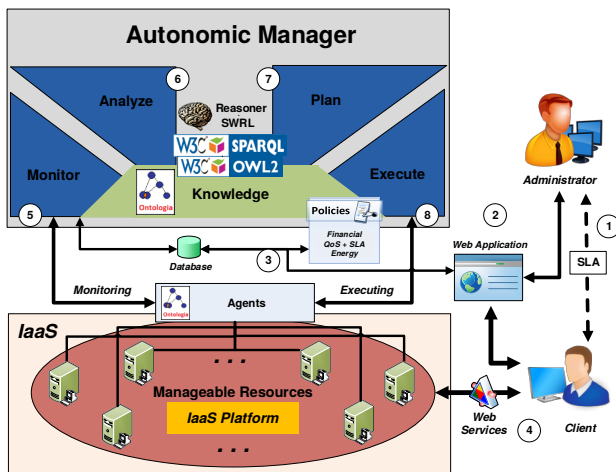
Fig. 2. Proposal Architecture
