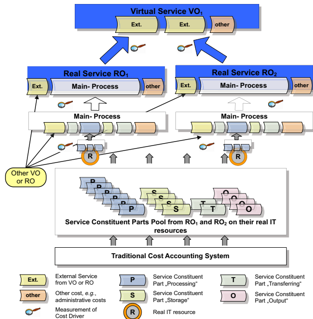
Figure 3: ABC Accounting Model for a DVO
