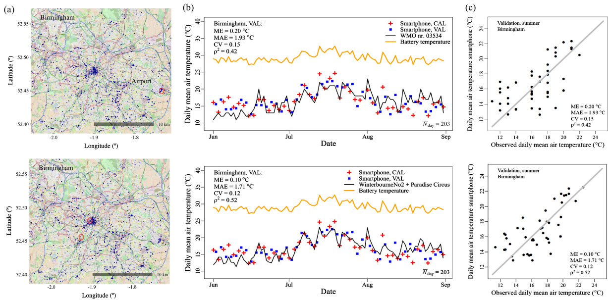
Figure 2. Estimation of air temperature from smart phone battery temperatures: comparison with data from (top) WMO Birmingham airport site (located just outside the city) and (bottom) two central Birmingham UKMO sites (which are located in the vicinity of a large number of battery readings): (a) Map of Birmingham (UK; © OpenStreetMap contributors; openstreetmap.org) showing locations of selected smart phone battery temperature readings (dots; blue in online) from 1 June to 31 August 2013 and location of WMO and UKMO weather stations (circles; red in online) (b) Time series of daily averaged observed and estimated air temperatures, as well as battery temperatures in Birmingham for same period. (c) Scatter plot of estimated daily air temperatures against observed daily air temperatures based on data from Birmingham for 1 June to 31 August 2013. Grey line is y = x line. ME denotes mean error (bias), MAE is mean absolute error, CV is coefficient of variation, \rho^2 is coefficient of determination. CAL and VAL stand for calibration and validation data set, respectively. WMO nr. is World Meteorological Organization station index number.
