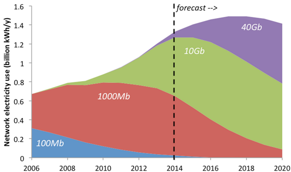
Figure 19. Total U.S. Data Center Network Equipment Electricity Consumption
