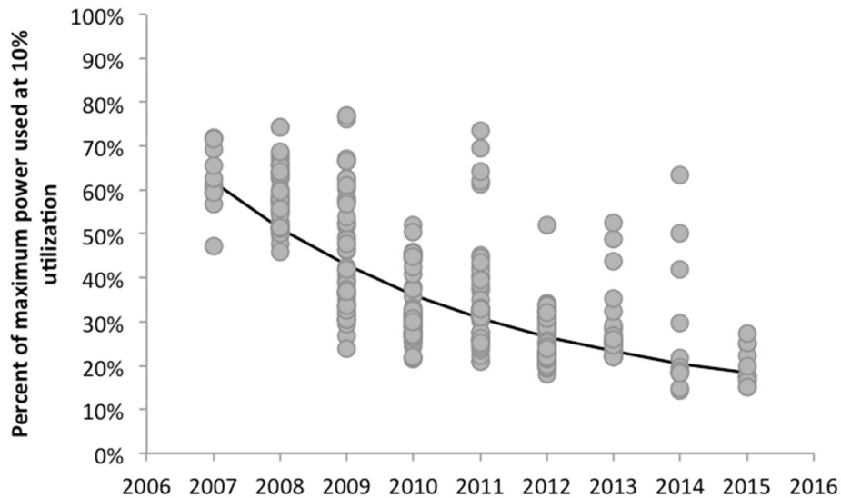
Figure 9. Dynamic Range of 1- and 2-Socket Servers in SPEC Database
