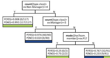
Fig. 2. Example RPT (pruned) to predict the successfulness of business projects
