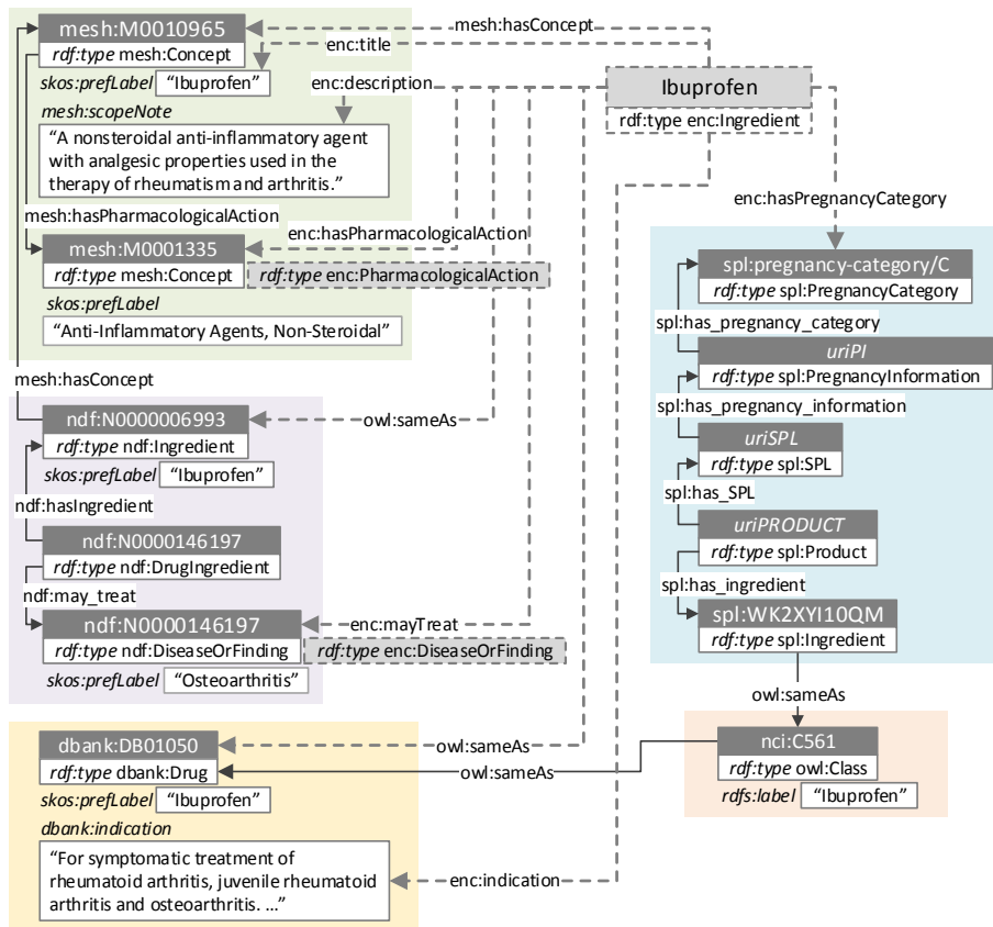
Fig. 2. Part of the triple store. The dashed lines represent the information in the data mart.
