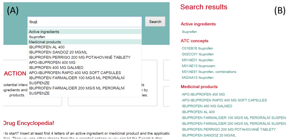
Fig. 3. Searching resources in the application data mart with Drug Encyclopedia
