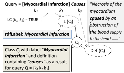
Fig. 2: Direct Parse
