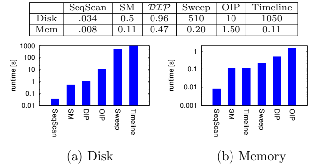
Fig. 28: Temporal join for the INFECTIOUS dataset in seconds.
