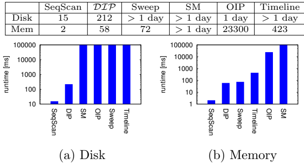
Fig. 27: Temporal join for the GREEND dataset in seconds.
