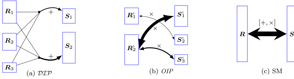
Fig. 11 DIP joins with linear cost (indicated by a + sign) many outer partitions with each inner partition. OIP joins with quadratic cost (indicated by a × sign) each outer partition with few inner partitions. Sort-merge backtracks without any guarantee about the complexity (i.e., ranges from linear to quadratic).
