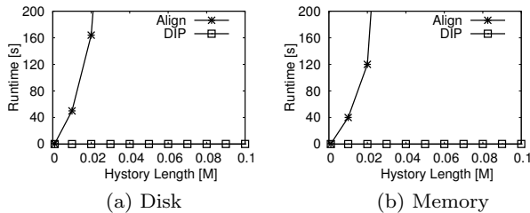
Fig. 23: Temporal anti-join.
