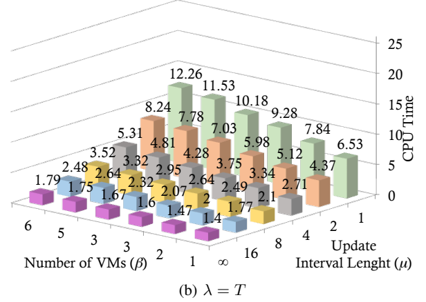
Fig. 2: CPU time consumed by OpenStack services dependent on the number of VMs ( \beta ) and the update interval ( \mu )
