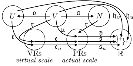
Fig. 1: Dependencies among the definitions of Section III
