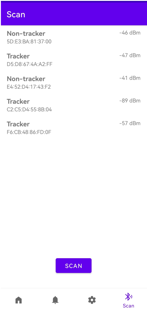
Figure 23: Integrated classification service in HomeScout.
