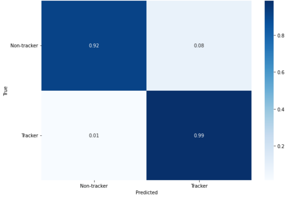
Figure 25: Confusion matrix of Random Forest classifier in feature-based prototype.
